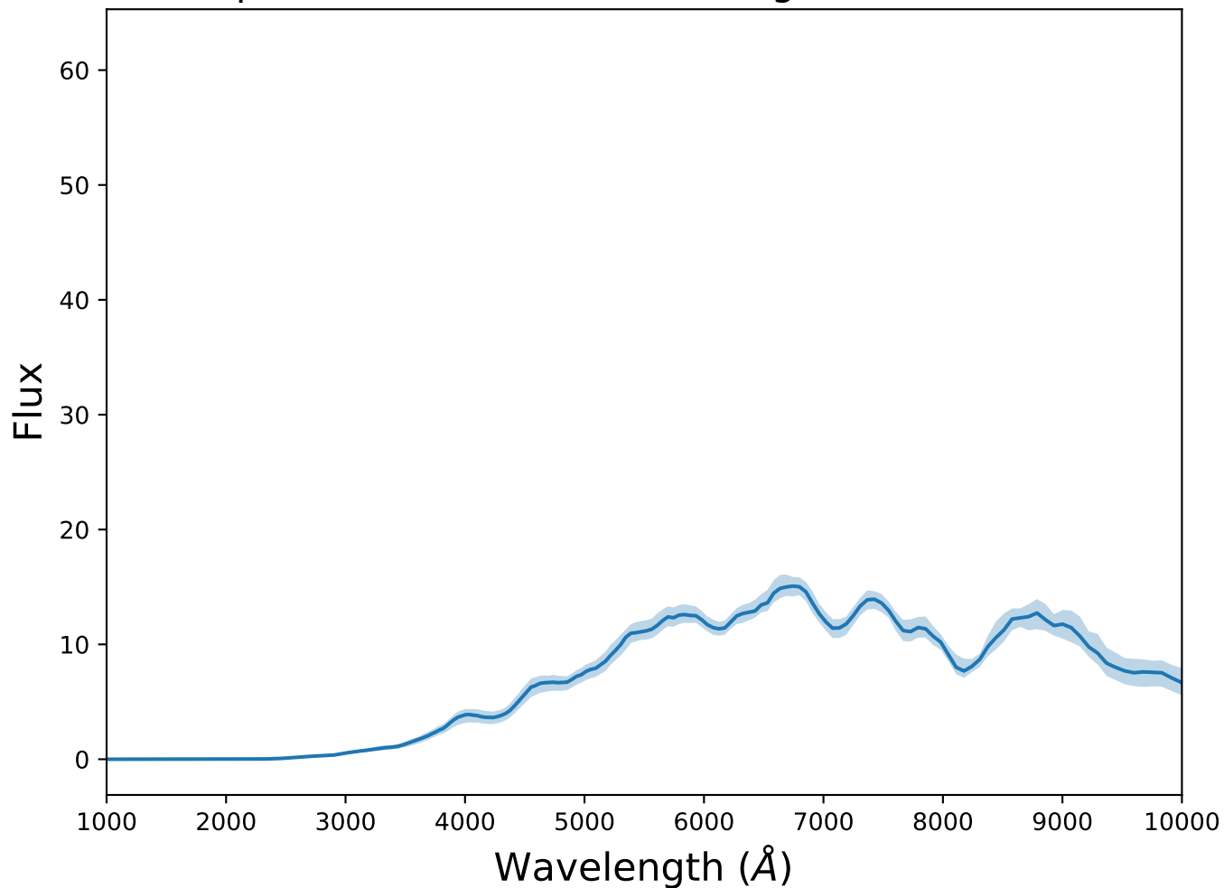
Spectrum 9 for transient 91bg-like at z=0.61
